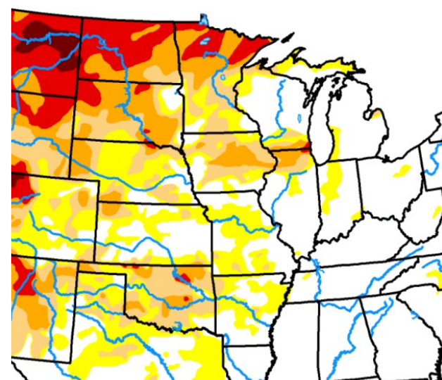
Figure 1. Drought-stressed areas on Sept. 28, 2021 Source: https://droughtmonitor.unl.edu/
